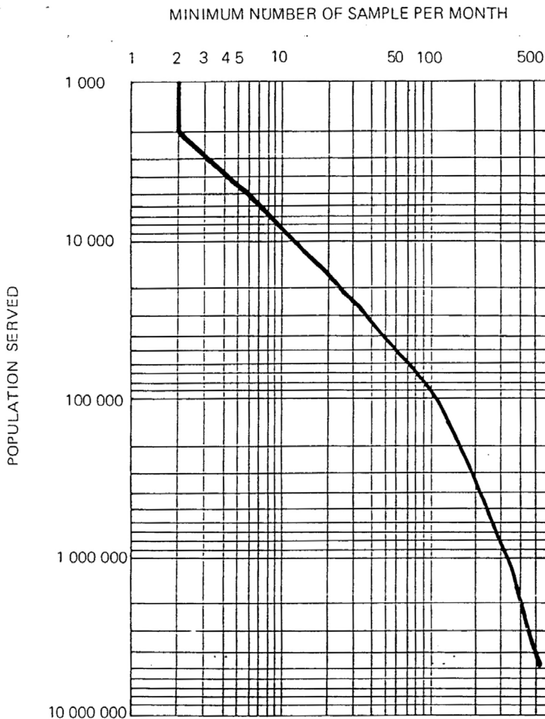
Fig. 1. Recommended minimum monthly samples per population served by water supply (bacteriological).
